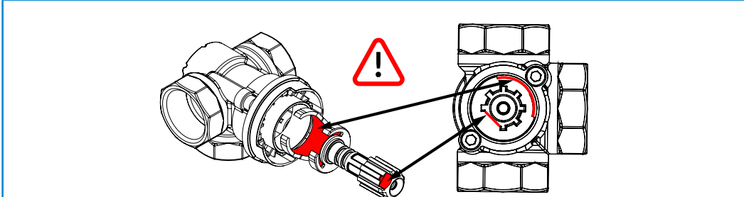
Fig. 2. Position of the closing element respect to the flattening on the adapter and valve spindle
