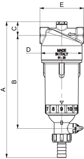
Fig. 4. Dimensions of the AWF water filters
