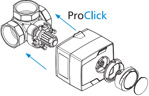
Rys. 5. System ProClick
