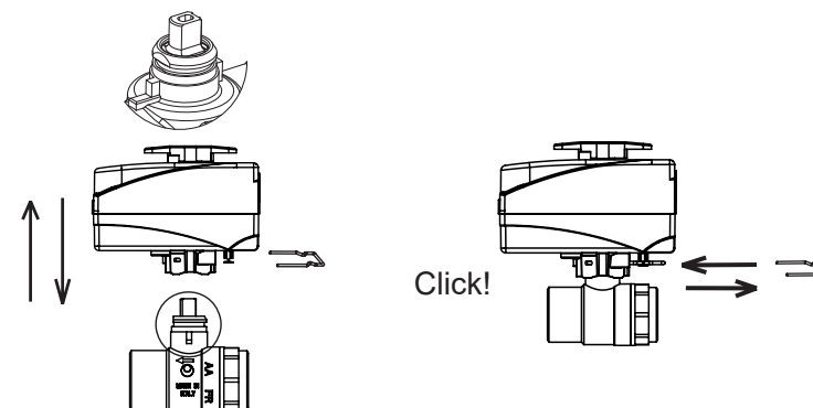
Fig. 3. Mounting of the actuator
