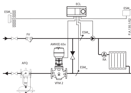
Direct-connected heating system
