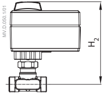
AMV 10, AMV 11 + VS 2 (DN 15-25)
