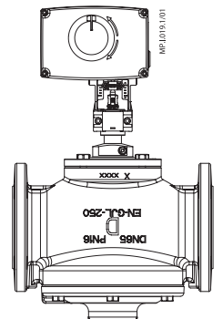
AMV(E) 438 SD + AHQM DN 50
