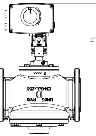
AMV(E) 438 SD + AHQM
